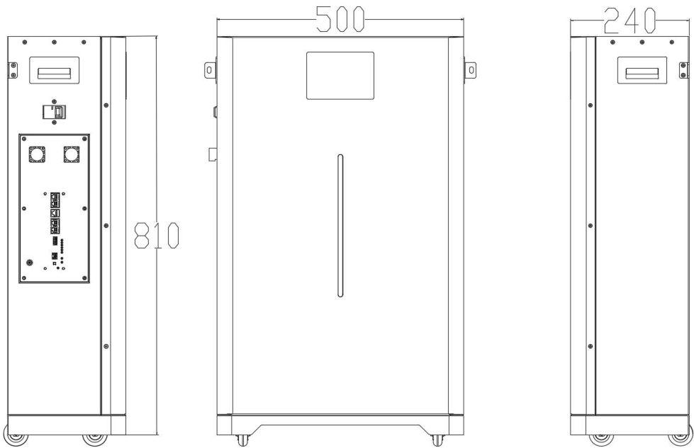
Dimension drawing
